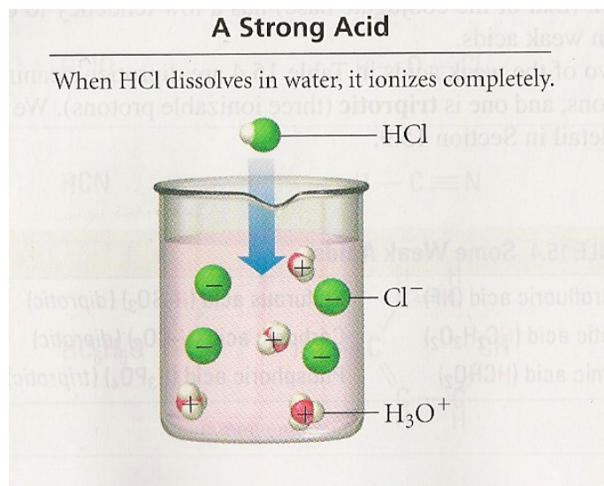
◀ FIGURE 15.4 Ionization of a Strong Acid When HCl dissolves in water, it completely ionizes to form H 3 O + and Cl - . The solution contains virtually no intact HCl.
