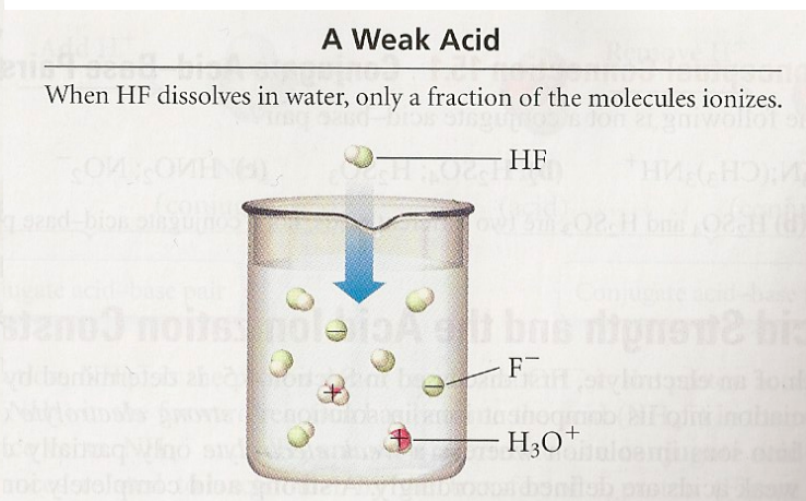
▶ FIGURE 15.5 Ionization of a Weak Acid When HF dissolves in water, only a fraction of the dissolved molecules ionize to form H 3 O + and F - . The solution contains many intact HF molecules.
