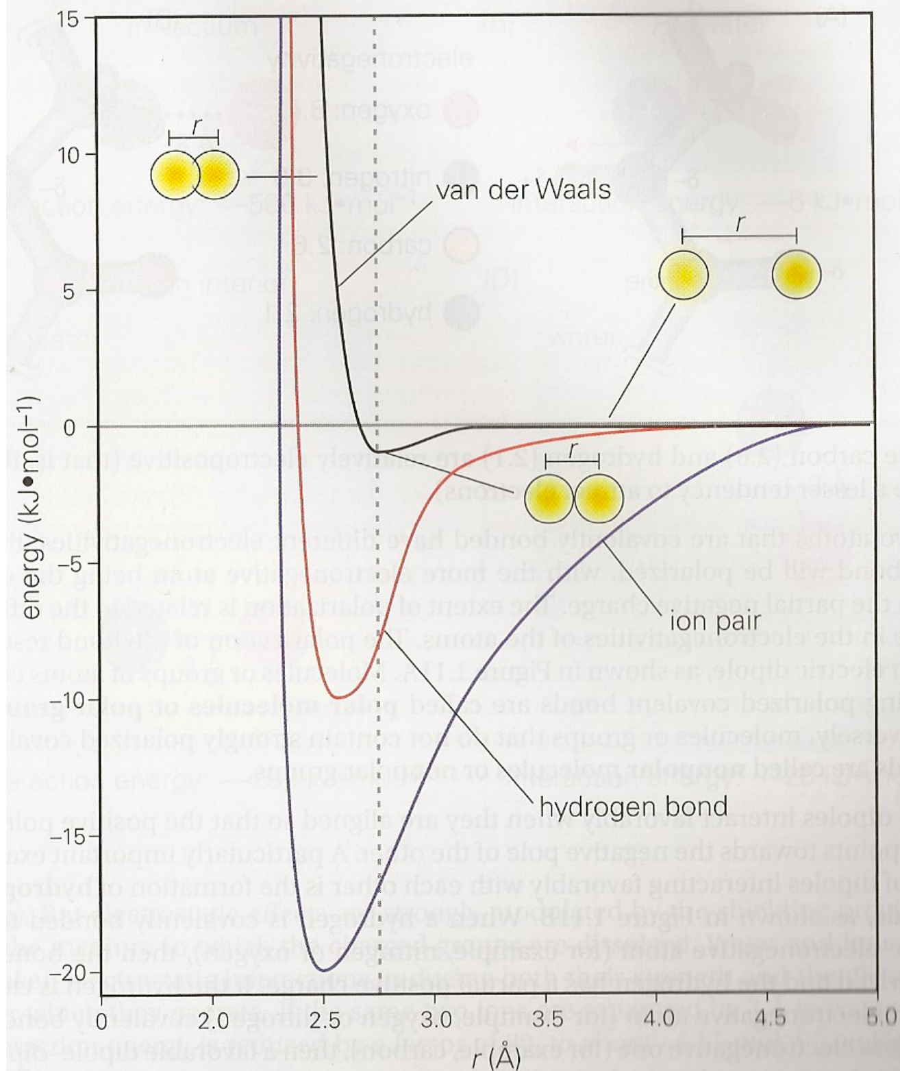
Figure 1.12 Graph of energy for a hydrogen bond. This graph shows how the energy of a \text{N}-\text{H}\cdots\text{O}-\text{C} hydrogen bond changes as the distance between the nitrogen and the oxygen atoms is varied (red). The energy for van der Waals and ion-pairing interactions between two atoms is also shown (black and blue; compare with Figures 1.6 and 1.9).
