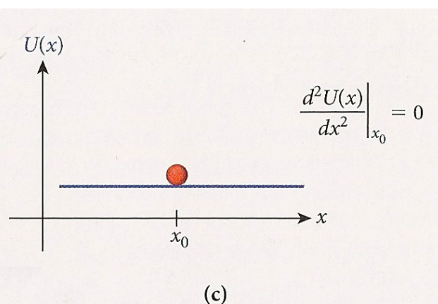
FIGURE 11.16 Local shape of the potential energy function at an equilibrium point: (a) stable equilibrium; (b) unstable equilibrium; (c) neutral equilibrium.
