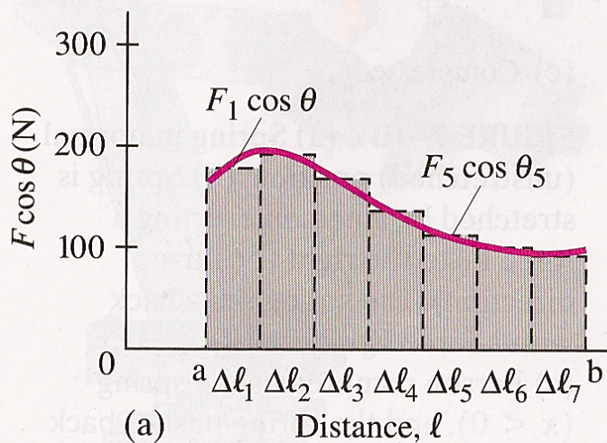
FIGURE 7-9 Work done by a force F is (a) approximately equal to the sum of the areas of the rectangles, (b) exactly equal to the area under the curve of F \cos \theta vs. \ell .
