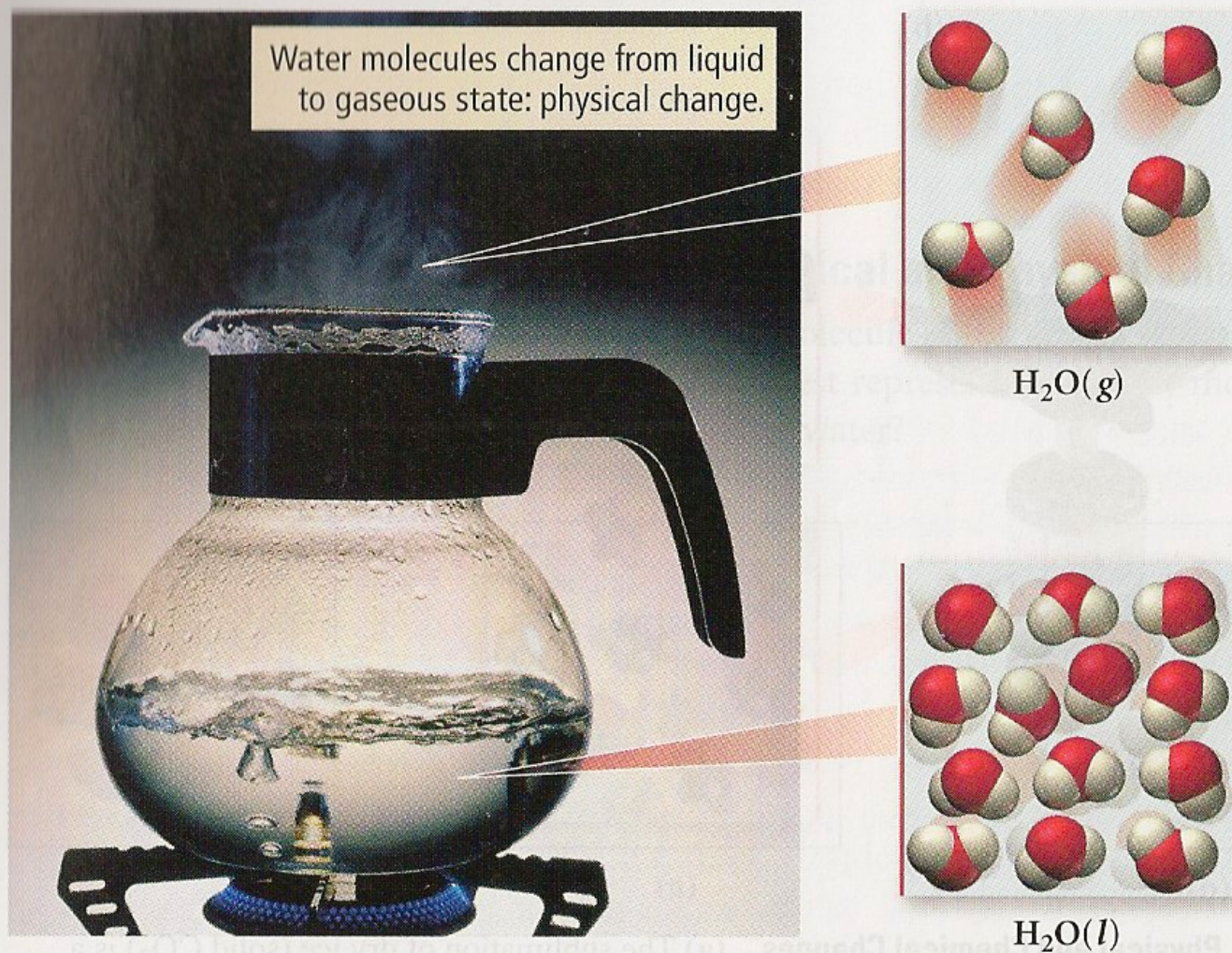
▲ FIGURE 1.7 Boiling, a Physical Change When water boils, it turns into a gas but does not alter its chemical identity—the water molecules are the same in both the liquid and gaseous states. Boiling is thus a physical change, and the boiling point of water is a physical property.
