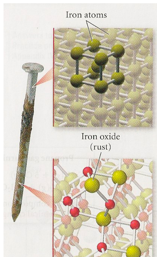
▲ FIGURE 1.8 Rusting, a Chemical Change When iron rusts, the iron atoms combine with oxygen atoms to form a different chemical substance, the compound iron oxide. Rusting is therefore a chemical change, and the tendency of iron to rust is a chemical property.
