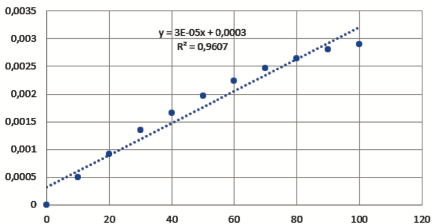
Graphe1 : x = f(t) x(mol)
